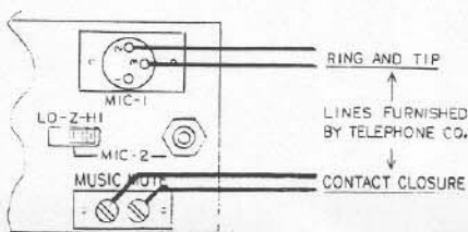
FIGURE 3: TELEPHONE INPUT CONNECTIONS USING TT-4 INPUT TRANSFORMER.
