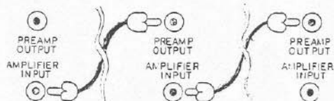
FIGURE 6: EITHER JACK MAY BE USED TO PARALLEL 810-100 AMPLIFIERS, ONLY IF INTERNAL JUMPER HAS NOT BEEN REMOVED.
